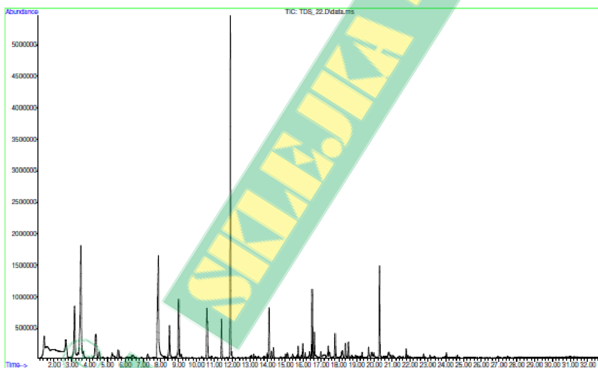
Chromatogram day 3
